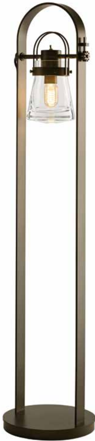
ERLENMEYER FLOOR LAMP • 247810 51" h x 11.3" dia • 11" rnd base • 29.5 lbs E26 Medium socket, 60W max, A19 bulb
